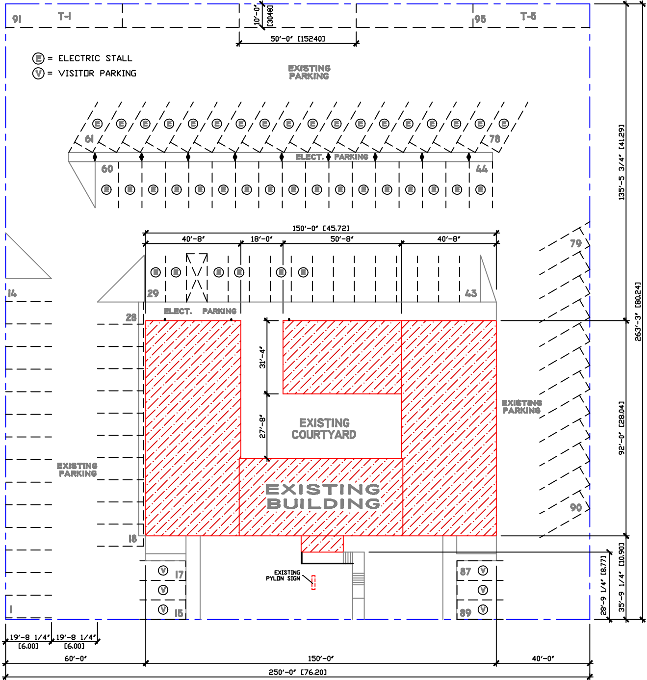
SITE PLAN (PARKING) SCALE 3/16"=1'-0"
